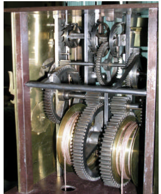
Note the two large crownwheels for timekeeping (Smaller crownwheel is for the alarm)
